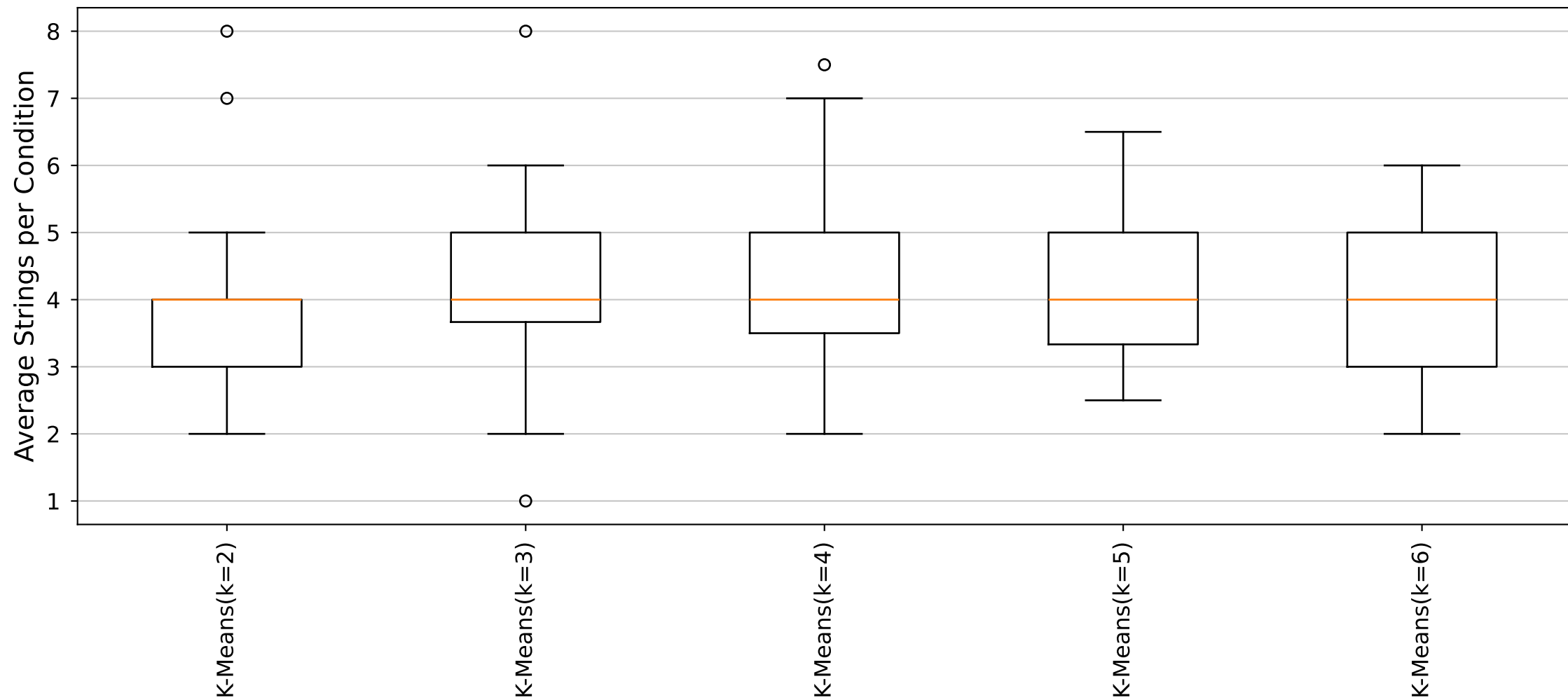
YARA Rules Average Strings per Condition Distribution (Cluster31_Size6 dataset)
